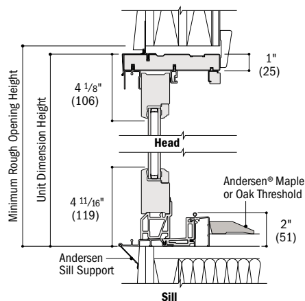
Vertical Section Stationary
