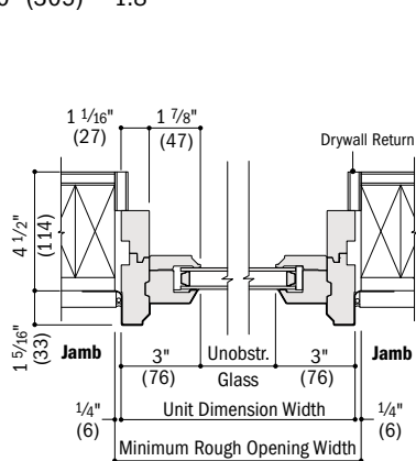
Horizontal Section
