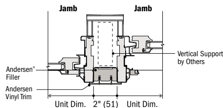
Horizontal Section Gliding and Gliding
