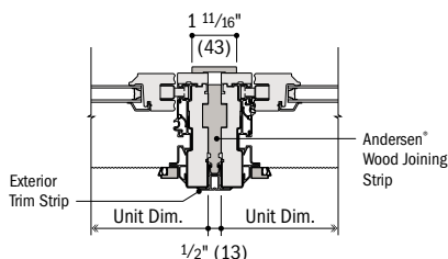
Horizontal Section
