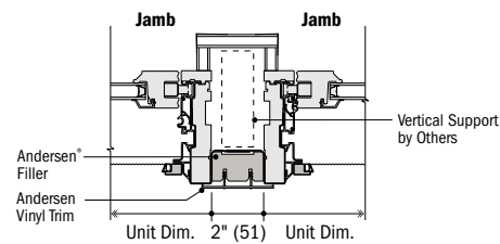
Horizontal Section
