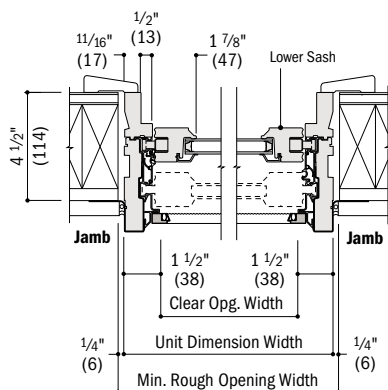
Horizontal Section
