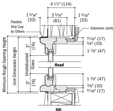
Vertical Section
