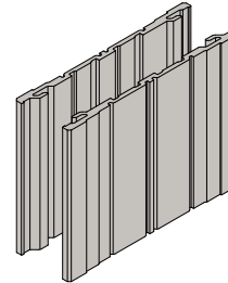
\frac{3}{4} " (19) x 7 \frac{3}{4} " (197) Fiberglass Joining Material For higher performance for 1-way and 2-way joining. Required for hinged inswing patio doors with 6 \frac{9}{16} " (167) base jamb depths.
