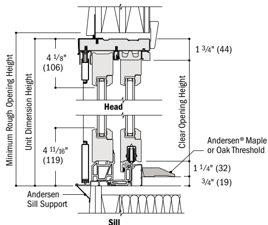
Vertical Section
