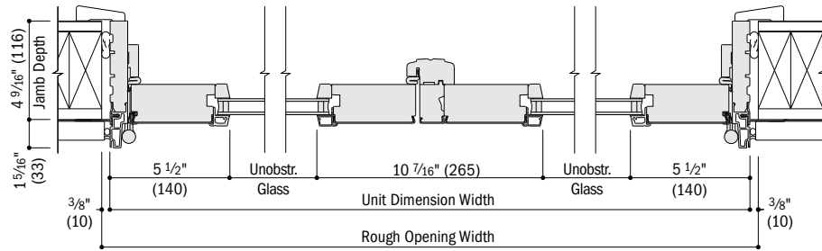
Horizontal Section Two-Panel
