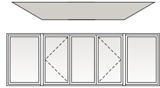
30BAY P3045-CW34-P3045
