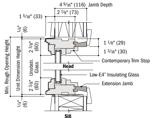
Vertical Section
