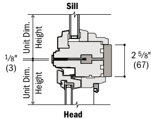
Vertical Section Picture (P) Over Casement
