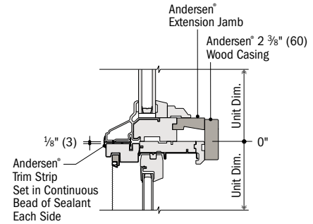
Vertical Section
