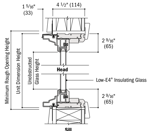
Vertical Section
