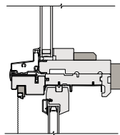
Vertical Section
