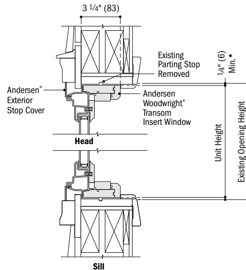
Vertical Section
