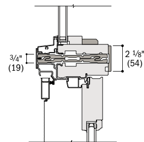
Vertical Section
