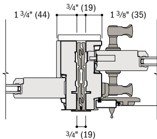
Horizontal Section Frenchwood® Gliding to Frenchwood Gliding
