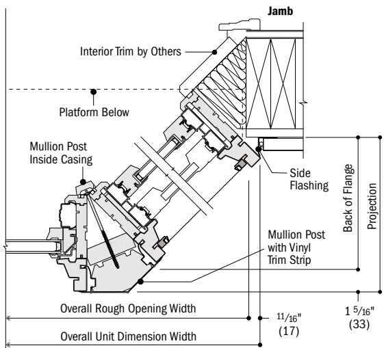
Horizontal Section
