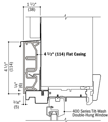
400 Series Tilt-Wash Double-Hung Window with 4 1/2" (114) Flat Casing
