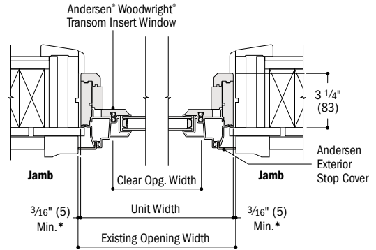
Horizontal Section
