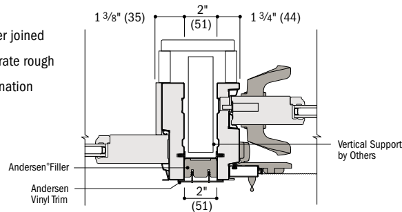
Horizontal Section Frenchwood® Gliding and Frenchwood Gliding
