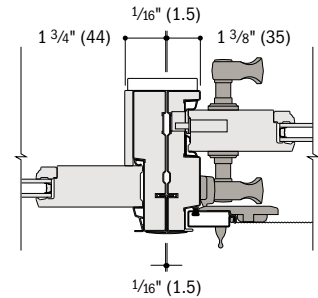
Horizontal Section Frenchwood® Gliding to Frenchwood Gliding
