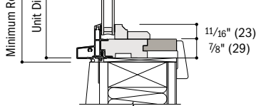
Sill
