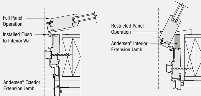
Jamb-Hinged Patio Door in 2 x 6 Wall Without Interior Extension Jamb
