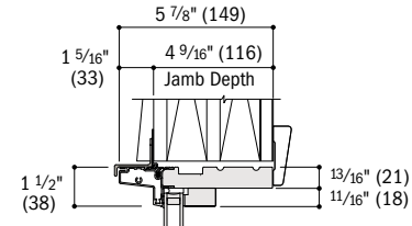
Lineal Head
