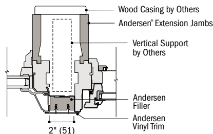
Horizontal Section
