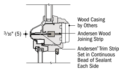
Vertical Section
