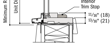
Sill
