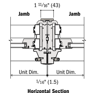
Horizontal Section
