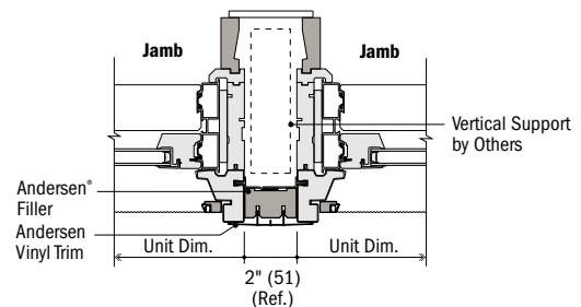
Horizontal Section
