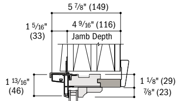
Lineal Head
