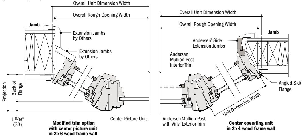
Horizontal Section
