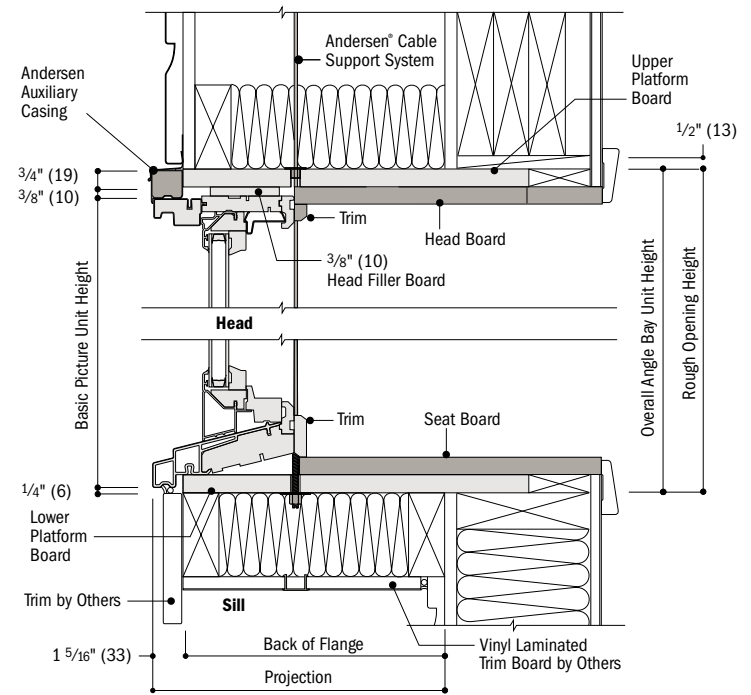
Vertical Section
