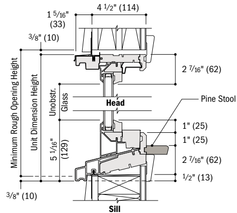
Vertical Section
