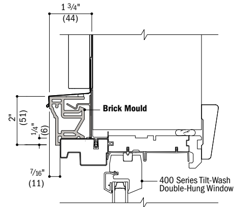
Vertical Section 400 Series Tilt-Wash Double-Hung Window with Brick Mould
