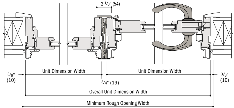
Horizontal Section Frenchwood® Patio Door Sidelight to Frenchwood Hinged Inswing Patio Door
