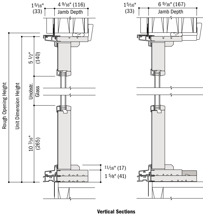
Vertical Sections
