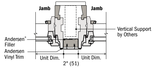
Horizontal Section Casement and Casement
