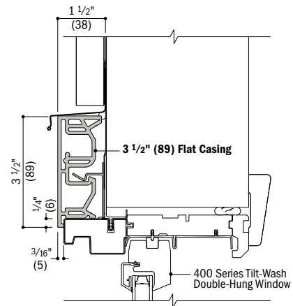
400 Series Tilt-Wash Double-Hung Window with 3 1/2" (89) Flat Casing
