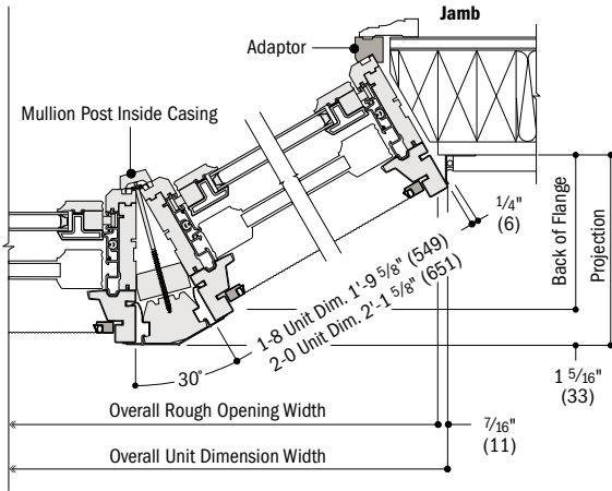
Horizontal Section
