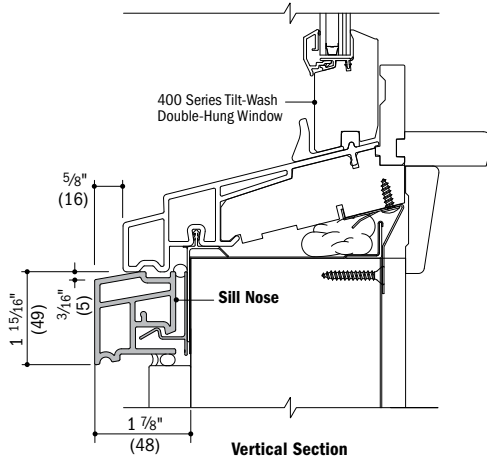
Vertical Section Sill Nose
