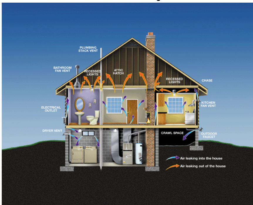
FIGURE 1: Location of Common Air Leakage Paths
