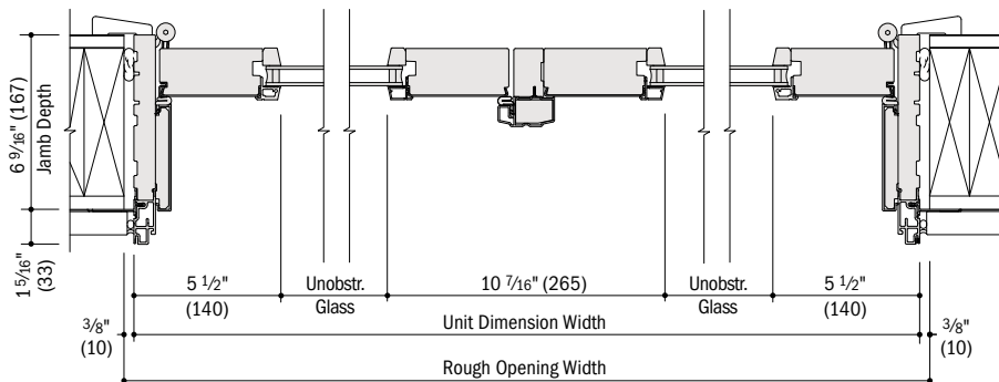
Horizontal Section
