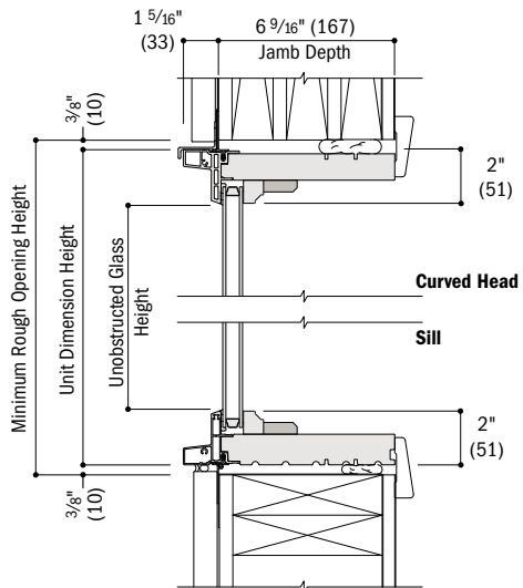
Vertical Section
