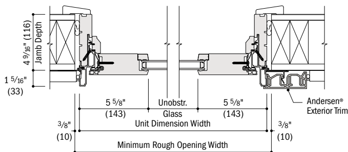
Horizontal Section Stationary (S), Contemporary Panel
