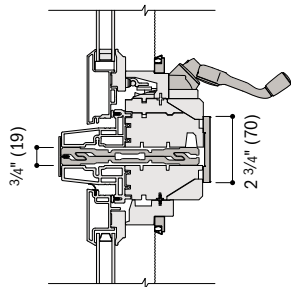
Casement/Awning Over Casement/Awning
