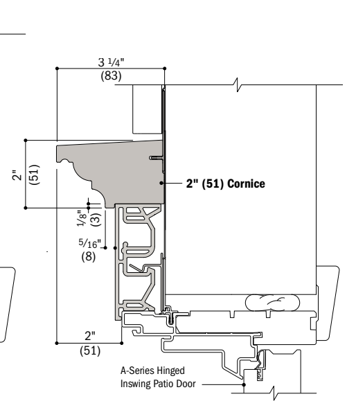
Vertical Section A-Series Hinged Inswing Patio Door with 2" (51) Cornice Over 3 1/2" (89) Flat Casing
