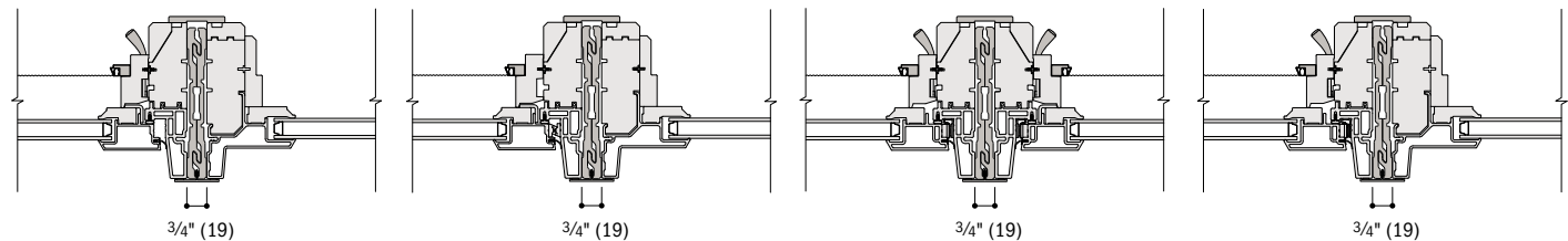
Casement to Picture Casement Lock Jamb
