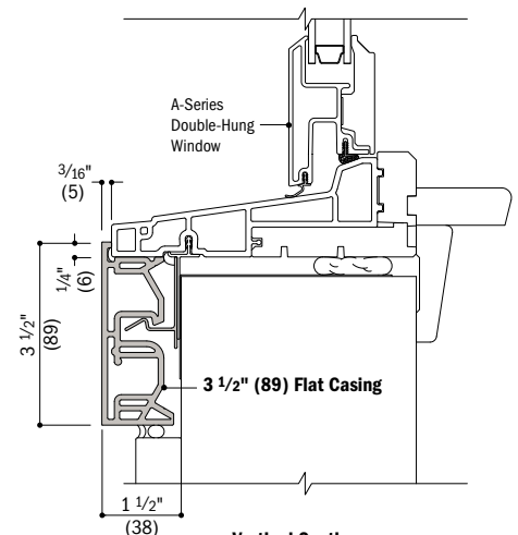
Vertical Section A-Series Double-Hung Window with 3 1/2" (89) Flat Casing at Sill
