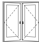
FWHID 6068 A P L R FWHICD Active Panel (panel used most often) Left Hinged Door Rough Opening Passive Panel Right Hinged Hinged Inswing Patio Door with Traditional (FWHID) or Contemporary (FWHICD) Panels
