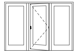
FWHID 9068 S A S R FWHICD Stationary Panel Stationary Panel Right Hinged Door Rough Opening Active Panel Hinged Inswing Patio Door with Traditional (FWHID) or Contemporary (FWHICD) Panels
