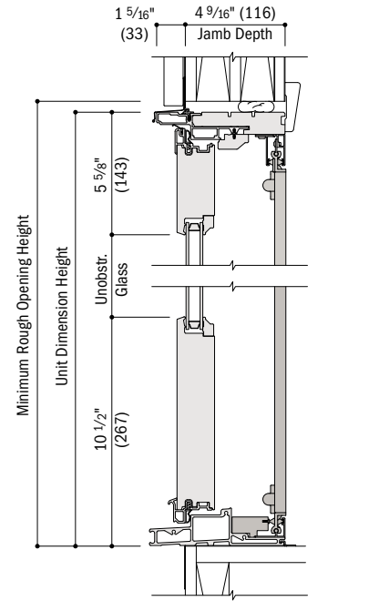
Vertical Section Active, Traditional Panel, Retractable Insect Screen
