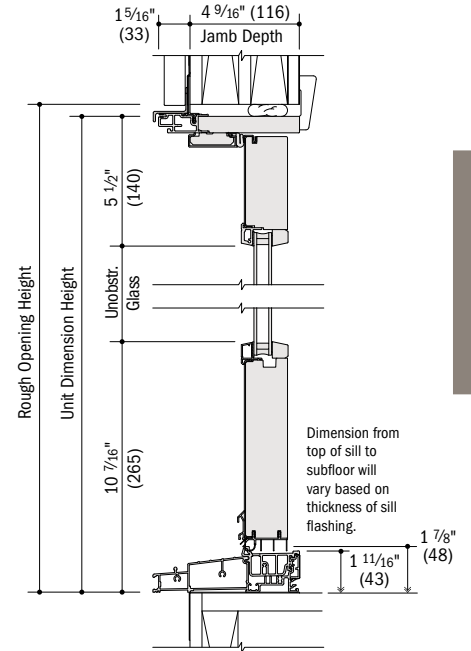
Vertical Section
