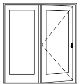
FWHID 6068 S A L FWHICD Stationary Panel Left Hinged Door Rough Opening Active Panel Hinged Inswing Patio Door with Traditional (FWHID) or Contemporary (FWHICD) Panels
