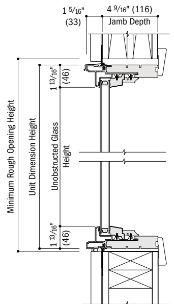
Vertical Section Transom and Sidelight Transoms
