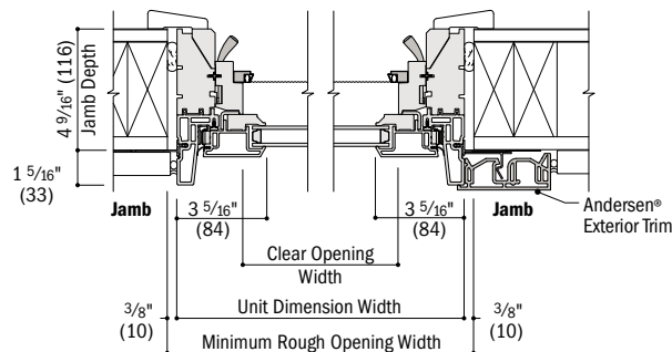
Horizontal Section
