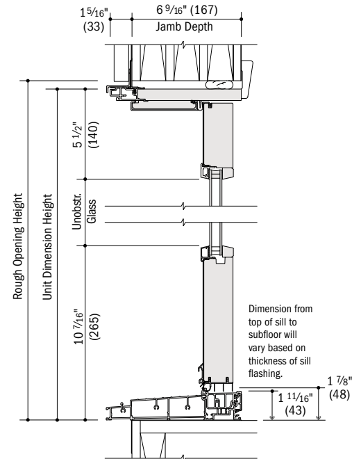
Vertical Section
