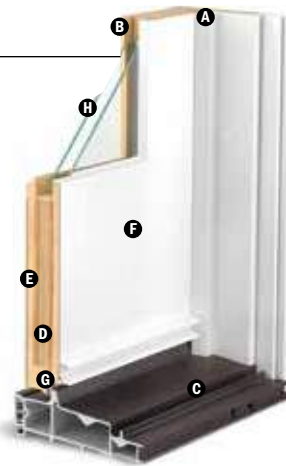
Traditional Panel
