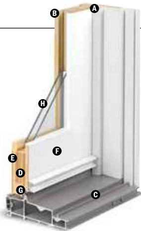
Contemporary Panel
