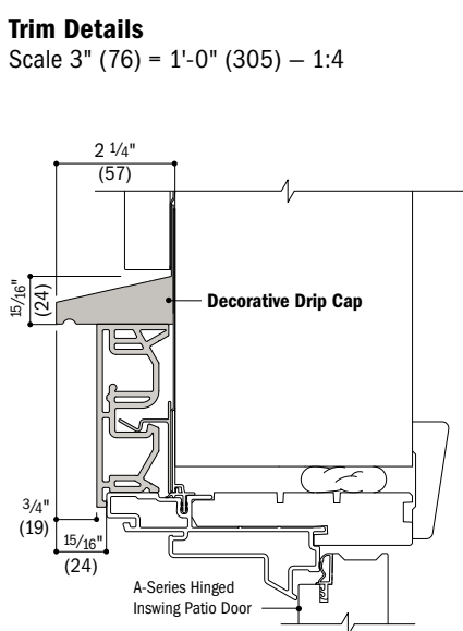
Vertical Section A-Series Hinged Inswing Patio Door with Decorative Drip Cap Over 3 1/2" (89) Flat Casing
