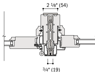
Hinge Jamb to Sidelight
