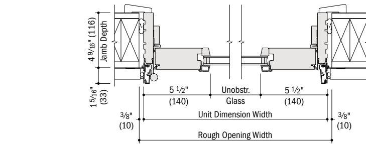
Horizontal Section
