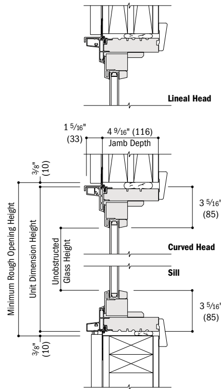
Vertical Section
