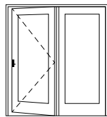
FWHID 6068 A S R FWHICD Active Panel Right Hinged Door Rough Opening Stationary Panel Hinged Inswing Patio Door with Traditional (FWHID) or Contemporary (FWHICD) Panels
