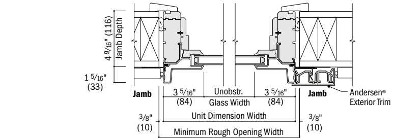
Horizontal Section
