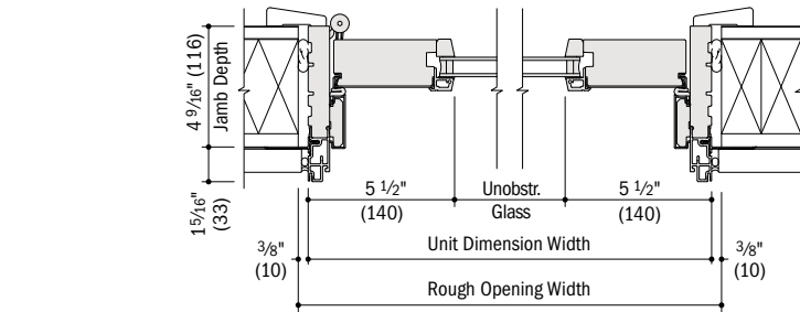
Horizontal Section
