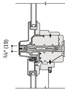
Fixed Transom Over Casement/Awning
