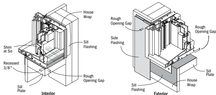
Example of window sill flashing in a membrane drainage system.
