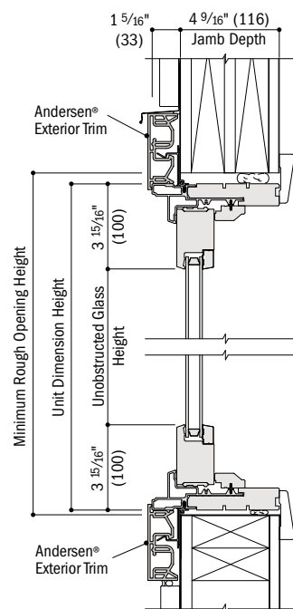
Vertical Section Transom and Sidelight Transom, Contemporary
