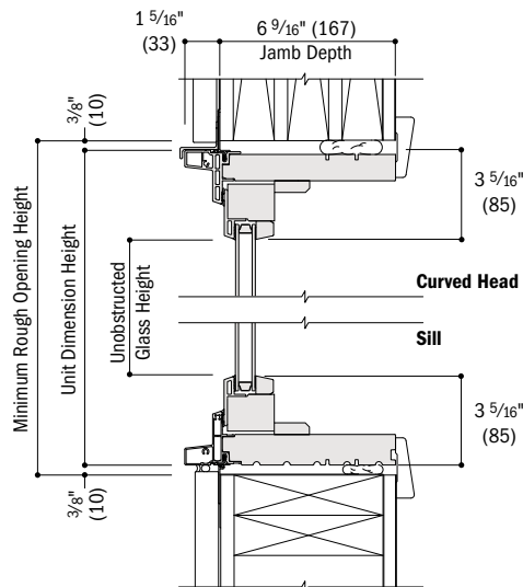
Vertical Section
