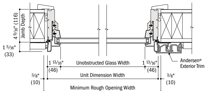
Horizontal Section Transom and Sidelight Transom, Contemporary
