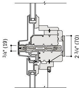
Picture Over Casement/Awning
