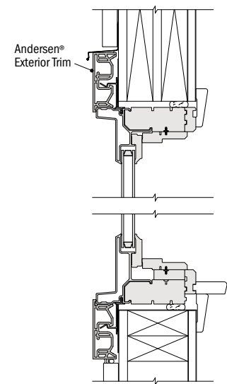
Vertical Section
