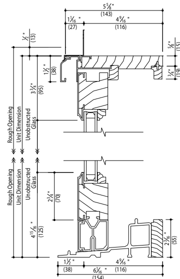
Vertical Section
