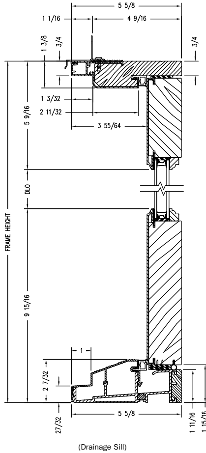
(Drainage Sill)
