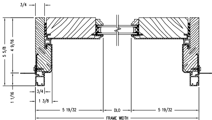
Horizontal Section
