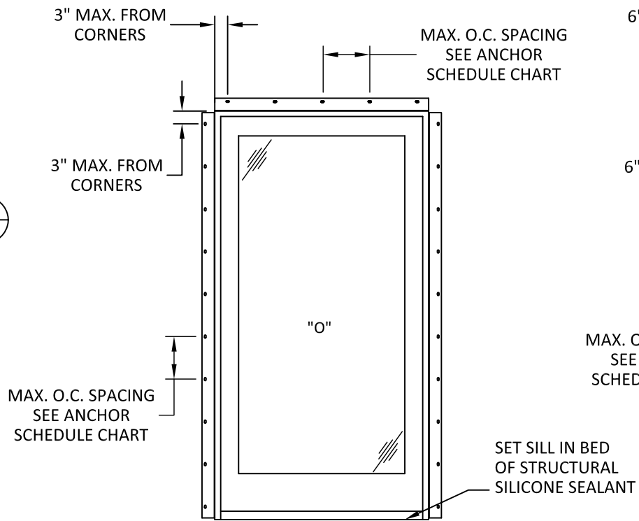
ANCHOR LAYOUT FIN INSTALLATION
