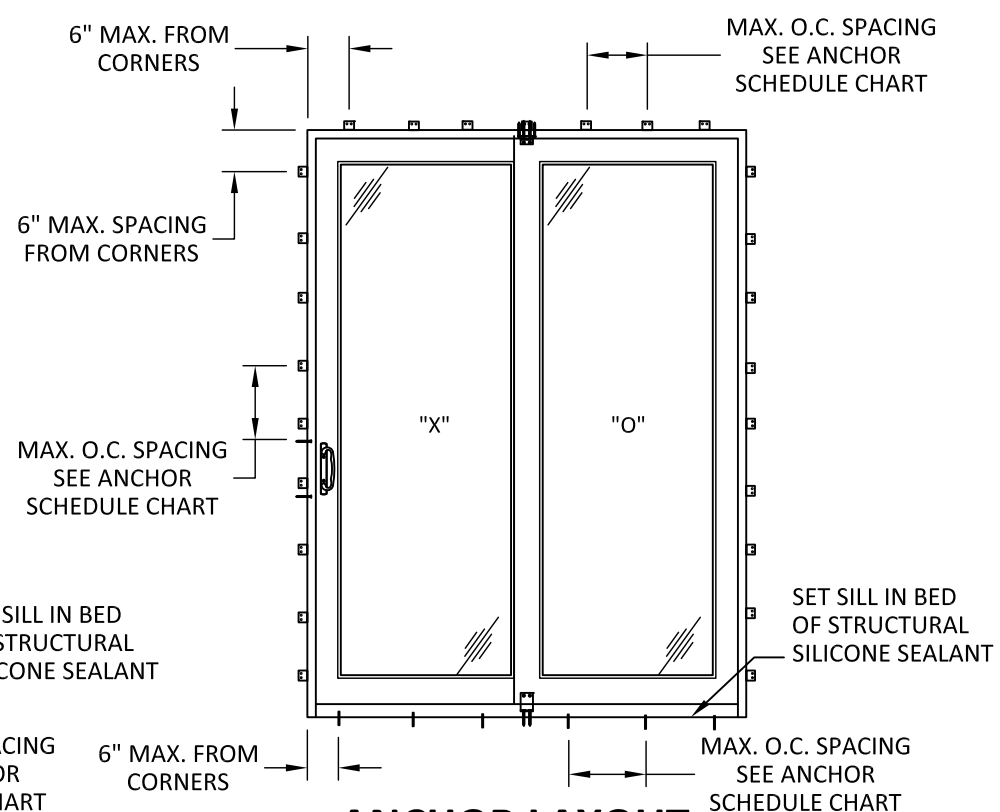
ANCHOR LAYOUT THROUGH STRAP INSTALLATION
