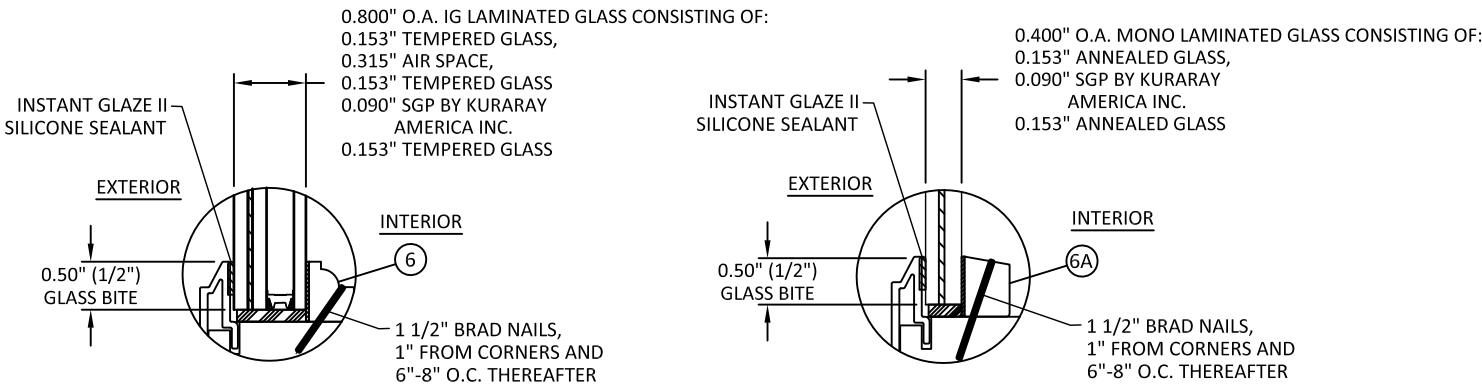
GLAZING DETAIL 1
