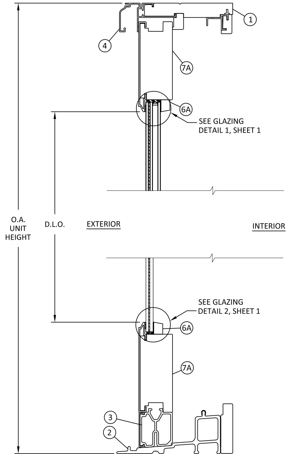
B 4 VERTICAL SECTION THROUGH
