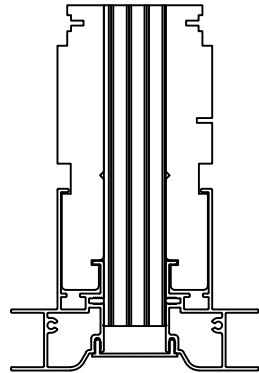
1" X 5 3/16" MULLION
