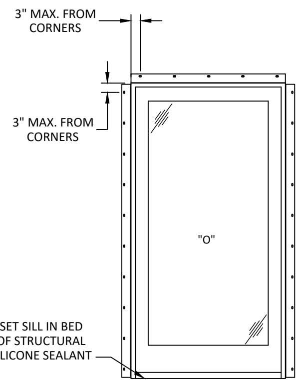
ANCHOR LAYOUT ALUMINUM FLANGE INSTALLATION
