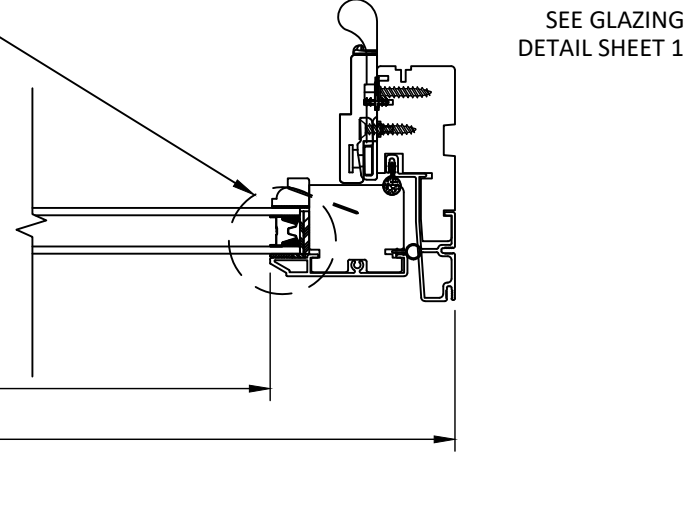
B 7 HORIZONTAL SECTION INSULATED GLASS
