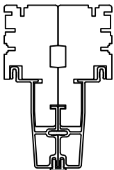
ZERO MULLION
