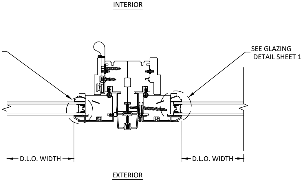
C 7 HORIZONTAL SECTION INSULATED GLASS ZERO MULLION
