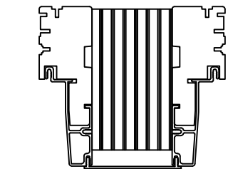
2" X 3-1/2" MULLION PROFILE
