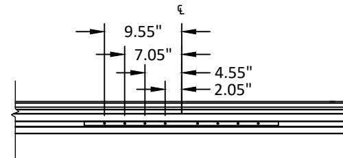
DETAIL 1
