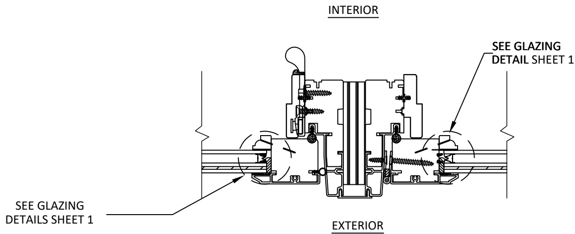
B 8 HORIZONTAL SECTION INSULATED GLASS 3/4" X 3-1/2" MULLION
