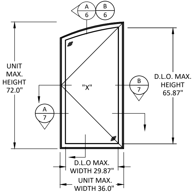
ELEVATION SINGLE UNIT
