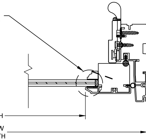
B 7 HORIZONTAL SECTION MONOLITHIC GLASS
