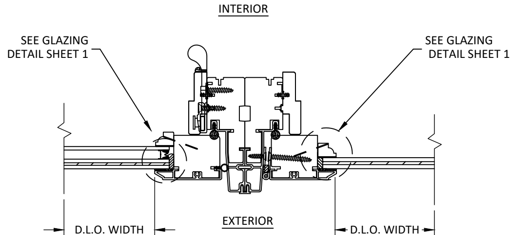
C 7 HORIZONTAL SECTION INSULATED/MONOLITHIC GLASS ZERO MULLION
