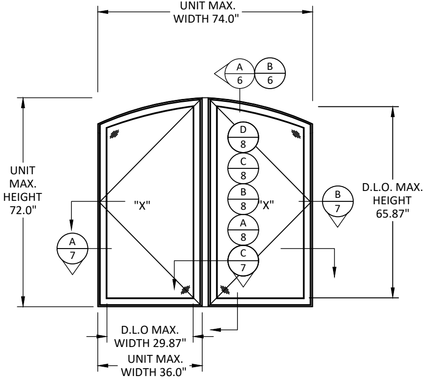
ELEVATION MULLED UNITS
