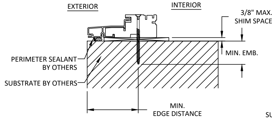
A 9 ANCHOR DETAIL THROUGH FRAME
