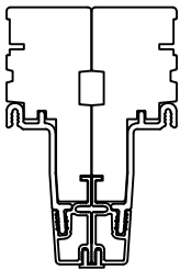
ZERO MULLION
