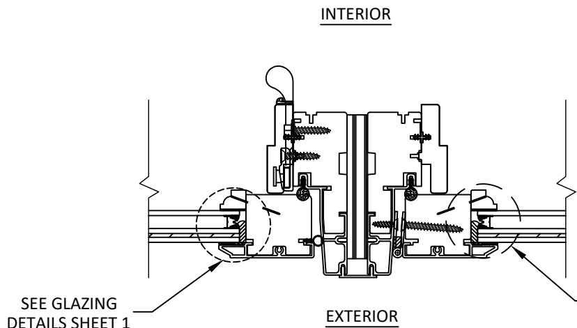
A 8 HORIZONTAL SECTION INSULATED GLASS 1/2" X 3-1/2" MULLION
