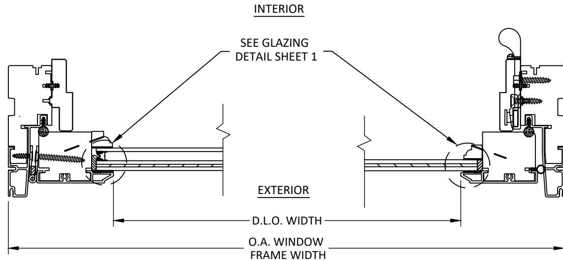
A 7 HORIZONTAL SECTION INSULATED GLASS
