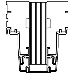
1" X 3-1/2" MULLION PROFILE
