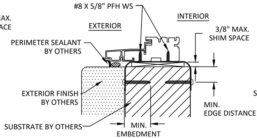
B 9 ANCHOR DETAIL STRAP ANCHOR
