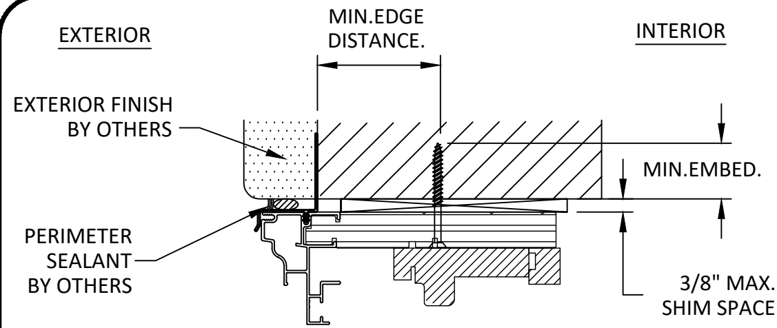
A 10 ANCHOR DETAILS THROUGH FRAME (HEAD AND SIDES ONLY)
