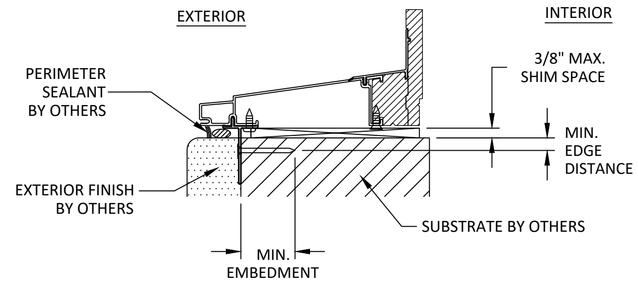
D 10 ANCHOR DETAILS THROUGH ALUMINUM FIN SILL
