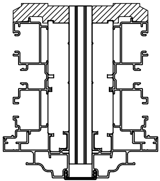
3/4" X 5 3/16" MULLION
