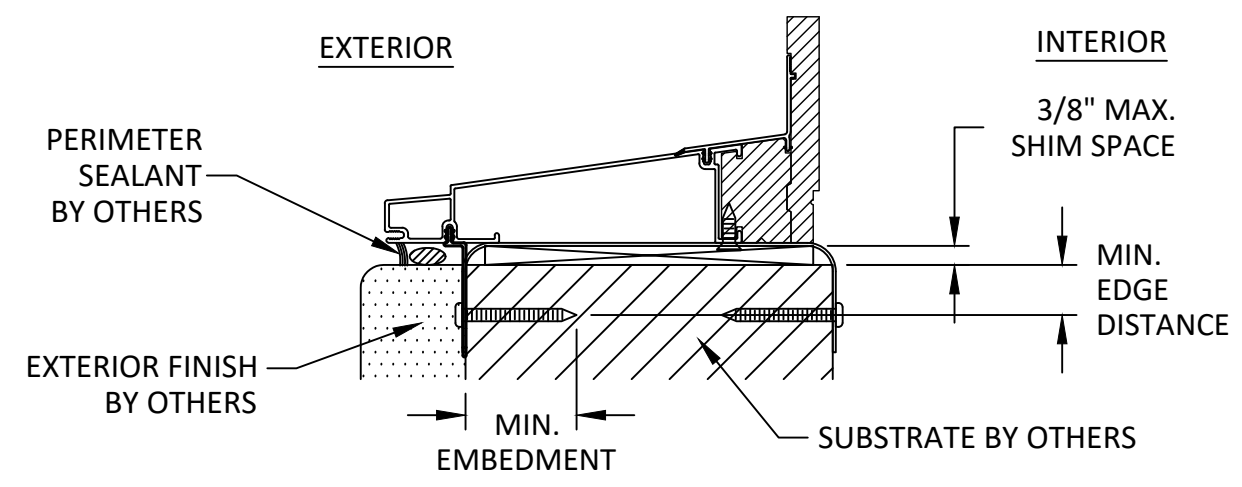
B 10 ANCHOR DETAILS STRAP ANCHOR (SILL, HEAD, AND SIDES)
