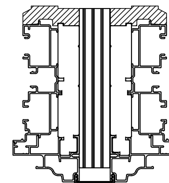
1" X 5 3/16" MULLION
