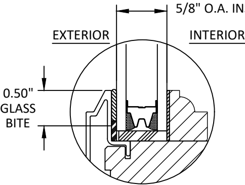
GLAZING DETAIL, G1 SHOWN WITH COLONIAL GLASS STOP
