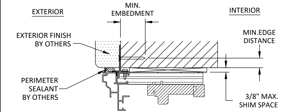
C 10 ANCHOR DETAILS THROUGH ALUMINUM FIN (HEAD AND SIDES ONLY)
