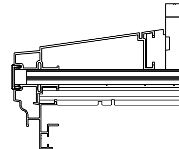
1/2" X 5 3/16" MULLION HORIZONTAL TRANSOM
