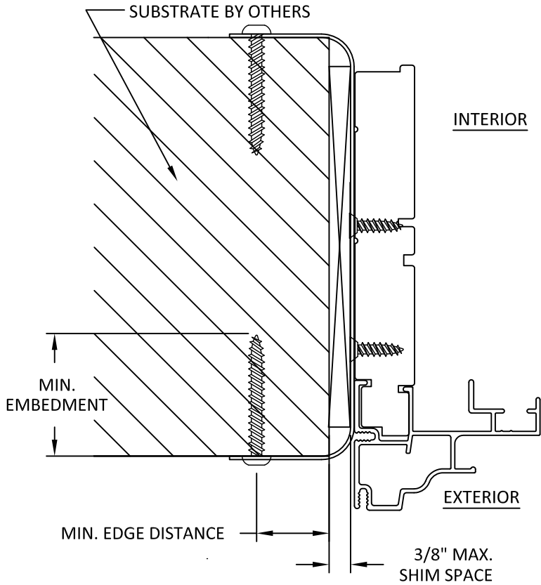
ANCHOR DETAIL STRAP ANCHOR (JAMB)
