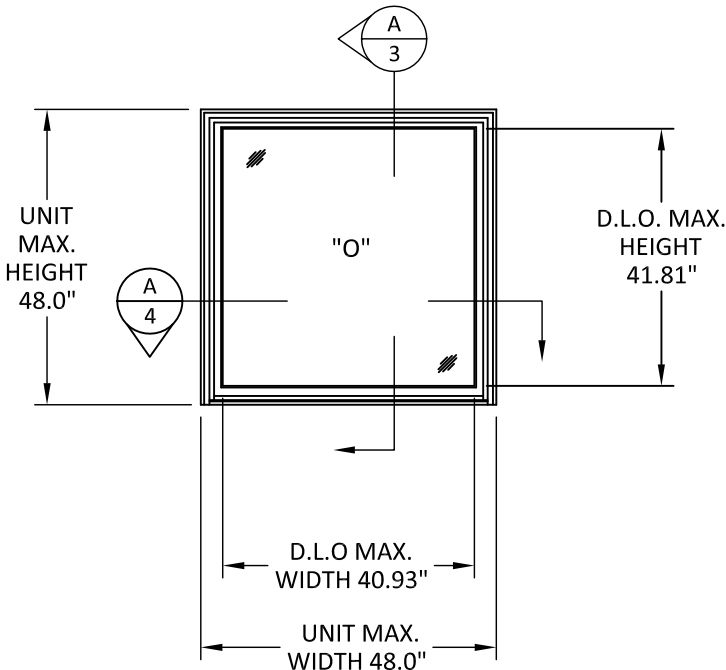
ELEVATION TRANSOM
