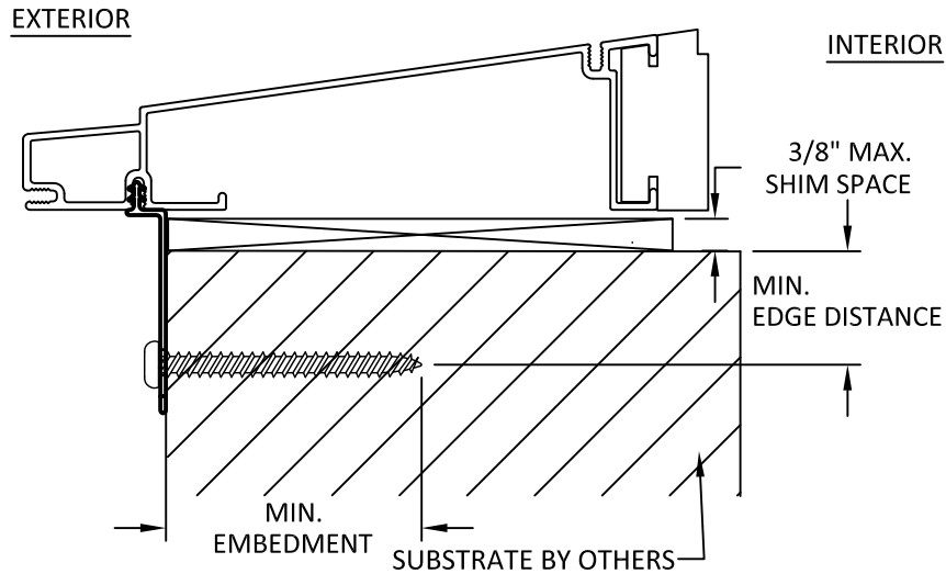
A 6 ANCHOR DETAIL VINYL - NAIL FIN (SILL)
