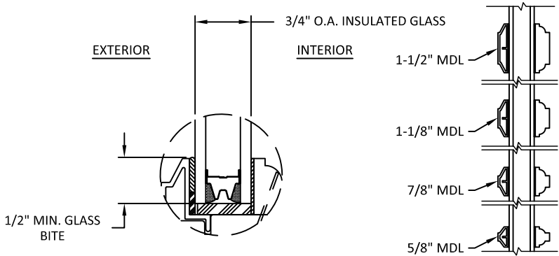
OPTIONAL MUNTIN BAR ATTACHMENT TO GLASS
