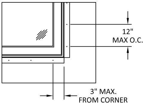
ANCHOR LAYOUT ALUMINUM NAIL FIN
