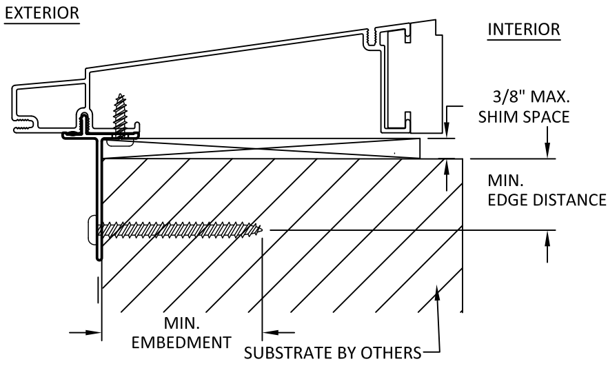
ANCHOR DETAIL ALUM - NAIL FIN (SILL)
