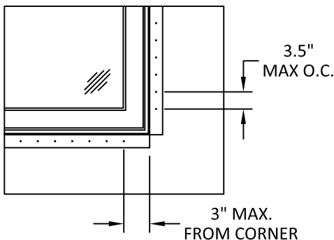
ANCHOR LAYOUT VINYL NAIL FIN
