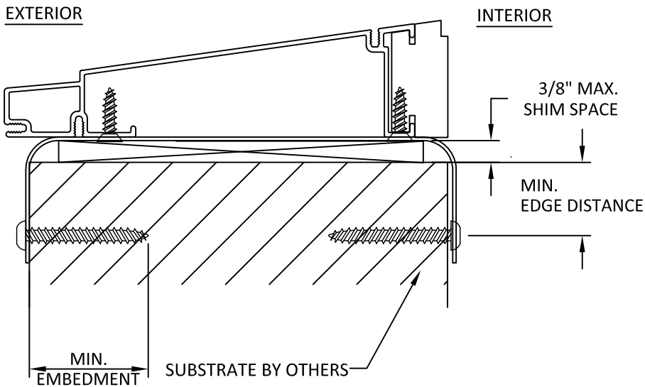
ANCHOR DETAIL STRAP ANCHOR (SILL)
