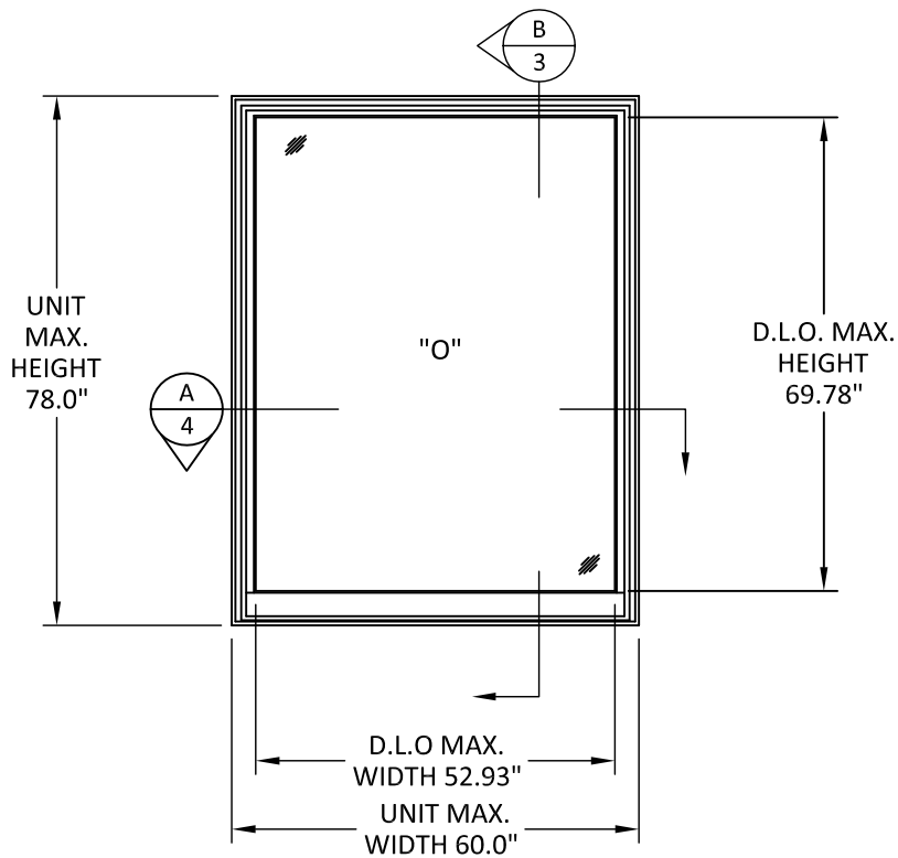
ELEVATION PICTURE WINDOW
