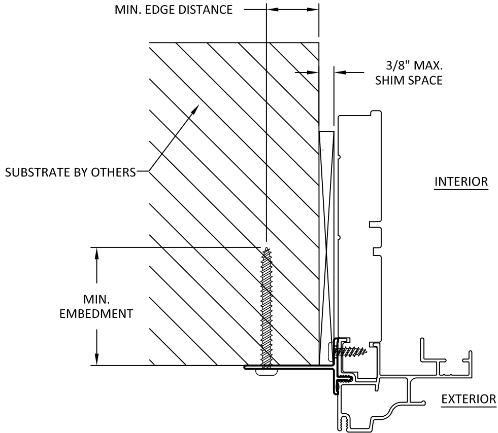
ANCHOR DETAIL ALUM - NAIL FIN (JAMB) HEAD HAS SIMILAR DETAIL
