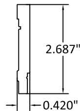
21 SILL STOP
