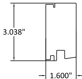
48 LOWER RAIL
