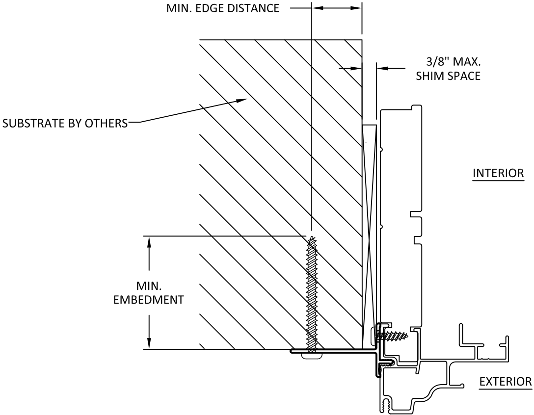
A 6 ANCHOR DETAIL NAIL FIN (JAMB)
