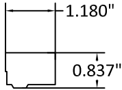
90 HEAD & SIDE STOP SUPPORT
