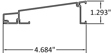
17 SASH COVER
