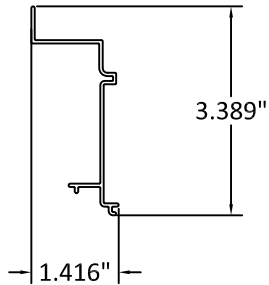
95 HEAD STOP EXTRUSION
