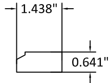
91 SIDE STOP SUPPORT
