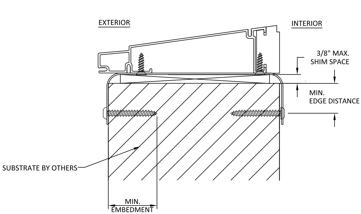
A 5 ANCHOR DETAIL STRAP ANCHOR (SILL)
