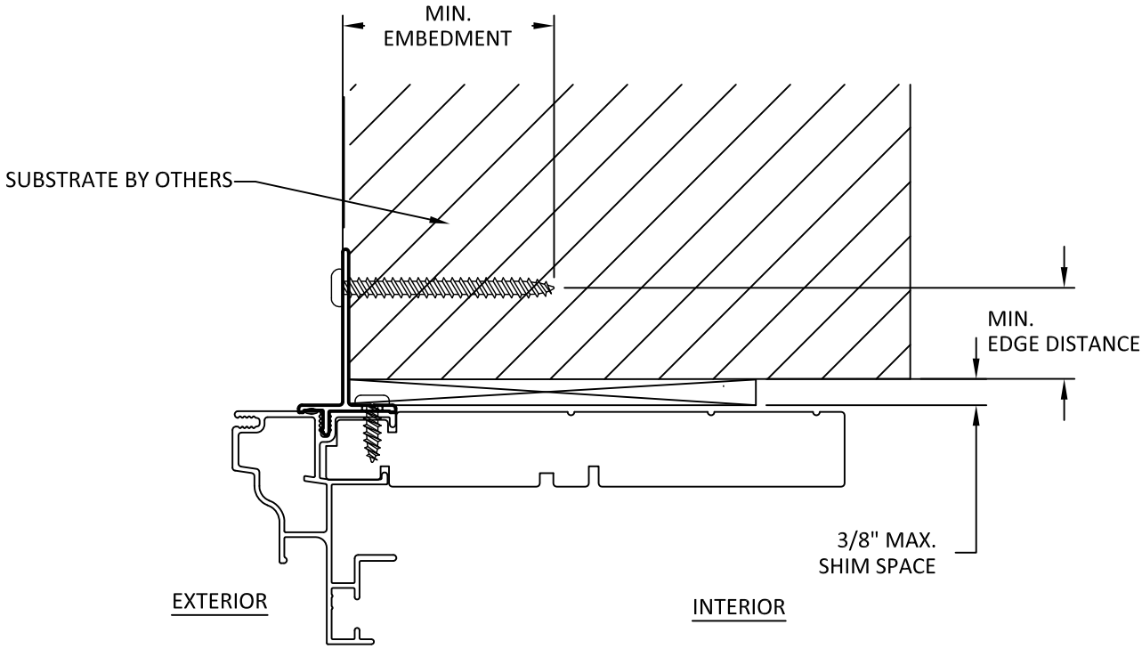
C 6 ANCHOR DETAIL NAIL FIN (HEAD)
