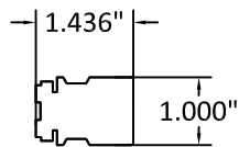
14 UPPER RAIL
