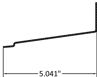
29 SILL PAD
