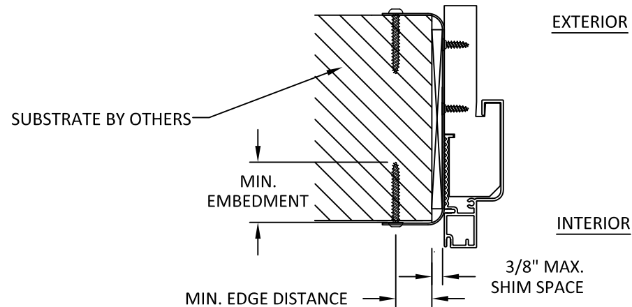
C 5 ANCHOR DETAIL STRAP ANCHOR (JAMB)
