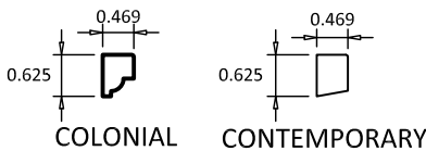
19 GLAZING STOP
