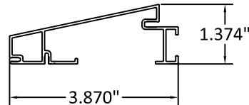
33 STRAP ANCHOR
