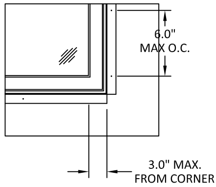
A/2 ANCHOR LAYOUT NAIL FIN
