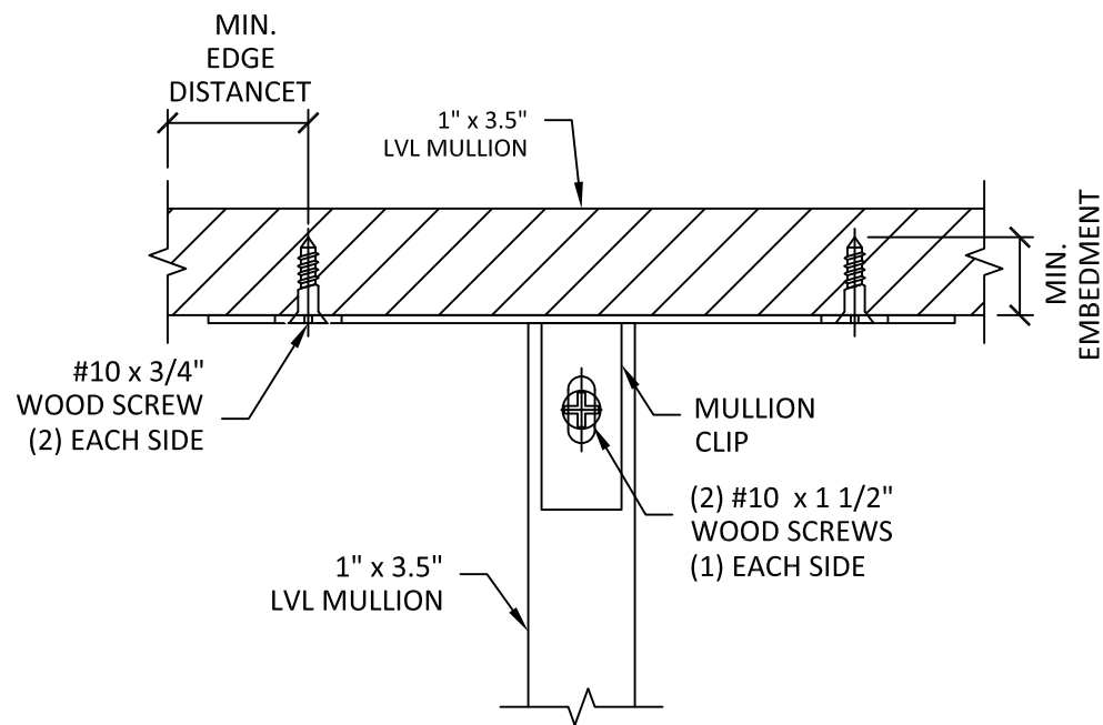
MULLION TO MULLION ANCHORING
