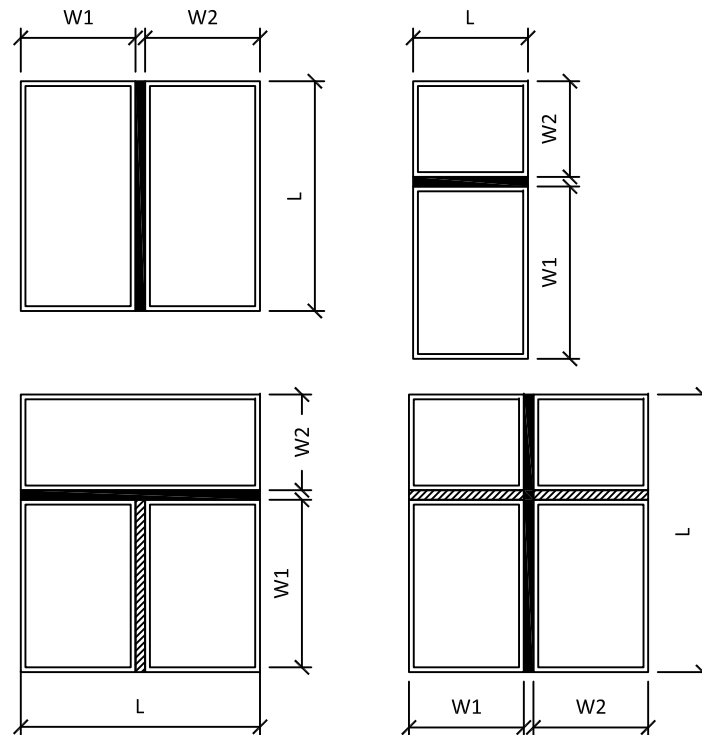
TYPICAL ELEVATIONS
