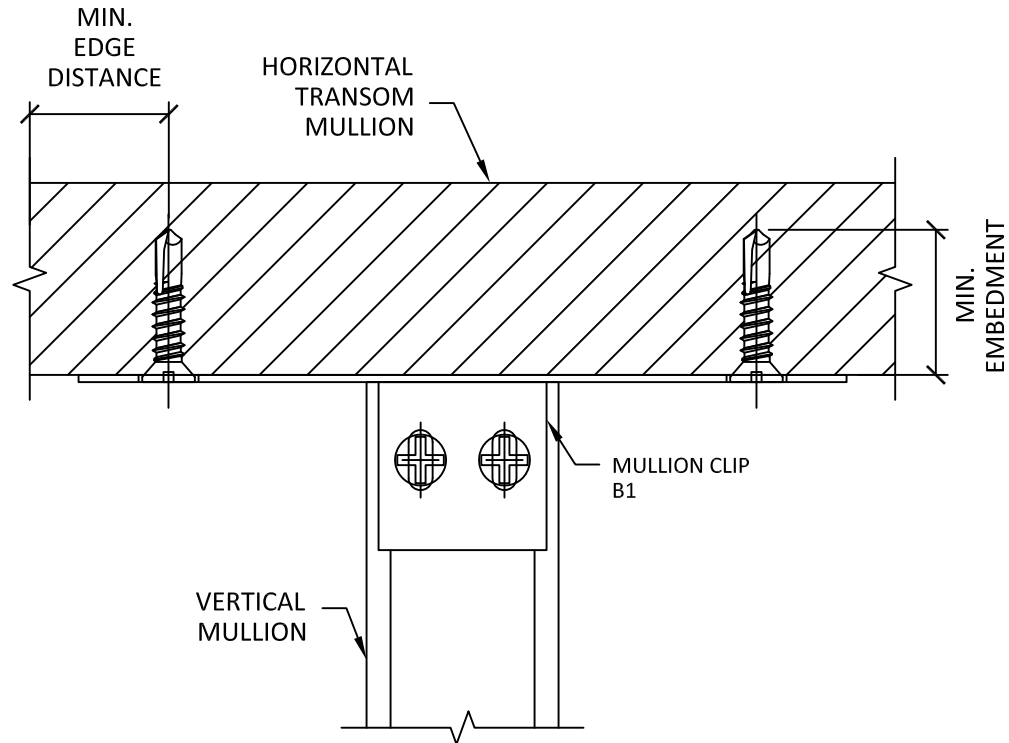
B 3 INSTALLATION DETAIL CLIP B1 INSTALLATION
