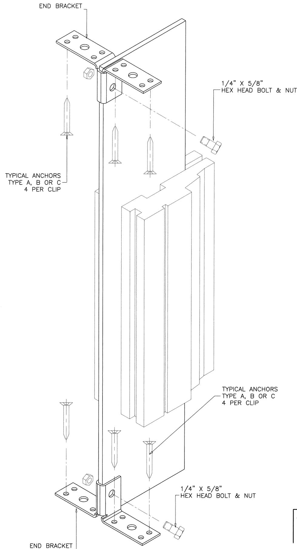
VERTICAL OR HORIZONTAL MULLION CONNECTION
