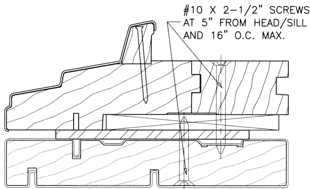
FLEXIFRAME/ARCH/SPRINGLINE TO FW GLIDING DOOR HORIZONTAL JOIN
