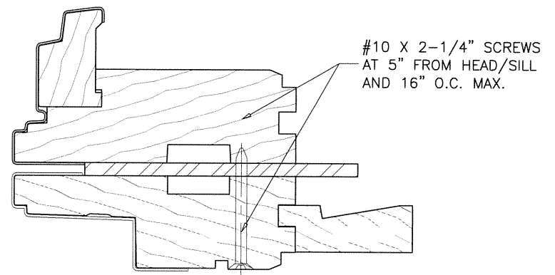
CASMT PICTURE WDW. TO CASEMENT HORIZONTAL JOIN
