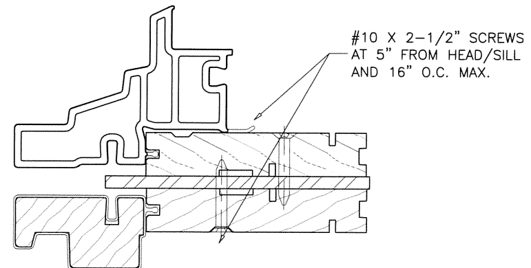
400 TW TO TW TRANSOM HORIZONTAL JOIN
