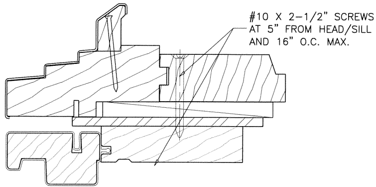
PSNL TO CIRCLE TOP--NL HORIZONTAL JOIN
