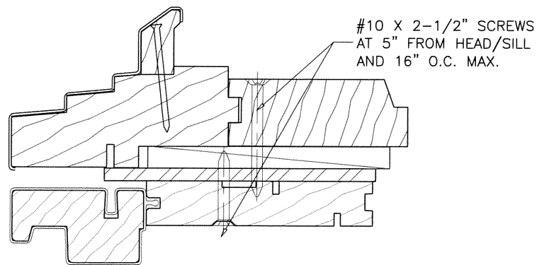
400 TW TO CIRCLE TOP--NL HORIZONTAL JOIN
