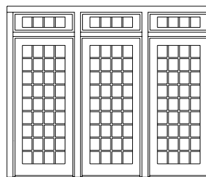
Single hinged patio doors with full-sized sidelights and transom windows
