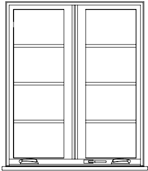
Window recessed in wall without head and jamb casing. Stool is simple rectangular profile with eased edge that projects beyond face of wall. Appropriate when window is recessed into wall.
