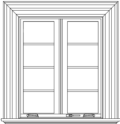
Head and jamb trim moulding with ogee and flat profile surrounded with backband. Stool with elliptical bull nose. Apron with common bed mould that is quarter round and cove profile. Appropriate when window is not recessed into wall.
