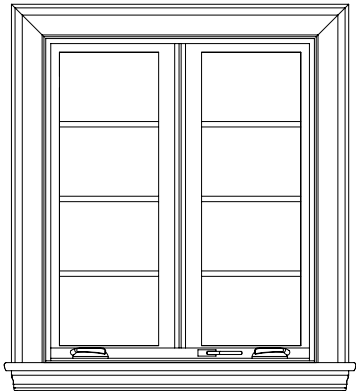
Beaded flat casing with backband for head and jambs. Stool with elliptical bull nose. Apron with ogee and bead profile. Appropriate when window is not recessed into wall.
